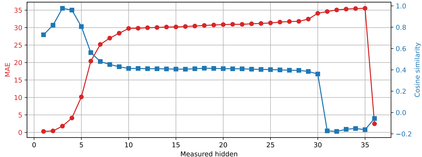
Qwen2.5-3B | Prompt 0 Spared layer 1 | Unquantized vs hybrid
