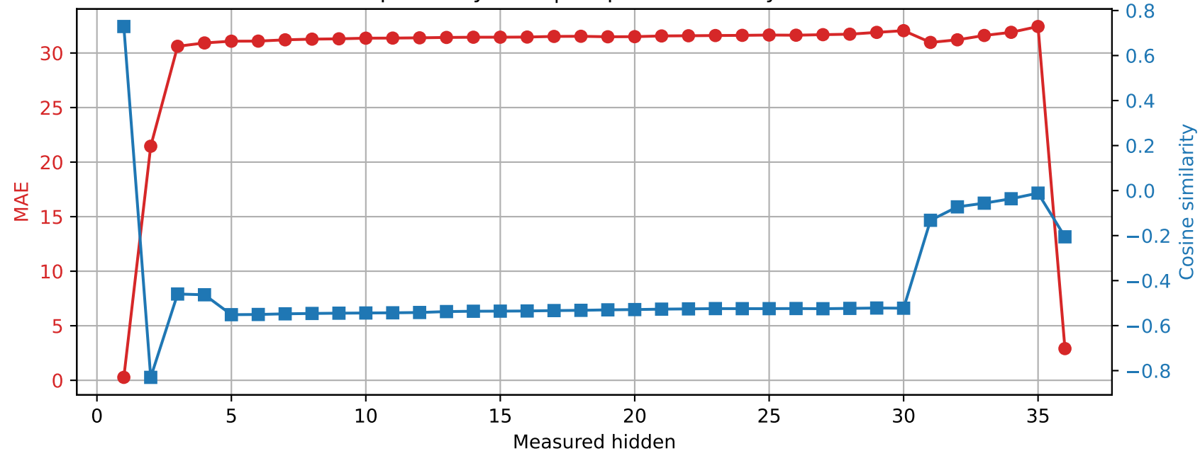
Qwen2.5-3B | Prompt 0 Spared layer 18 | Unquantized vs hybrid
