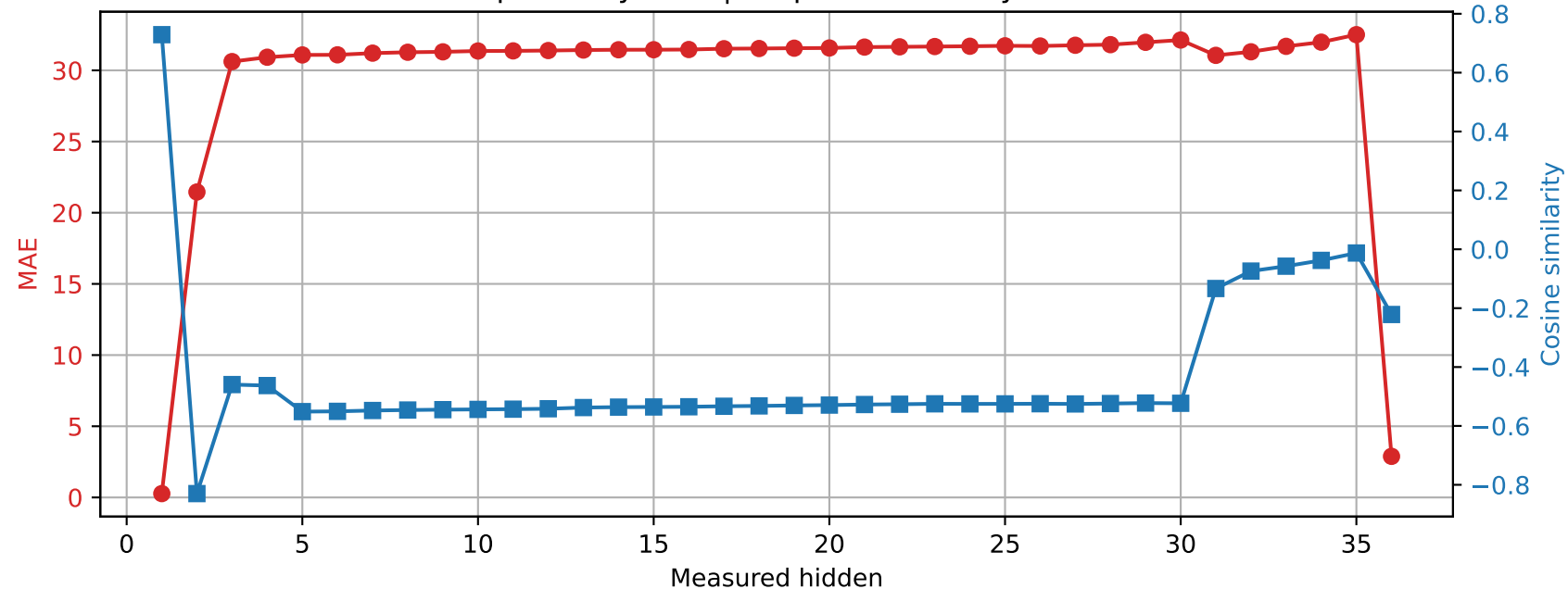
Qwen2.5-3B | Prompt 0 Spared layer 35 | Unquantized vs hybrid
