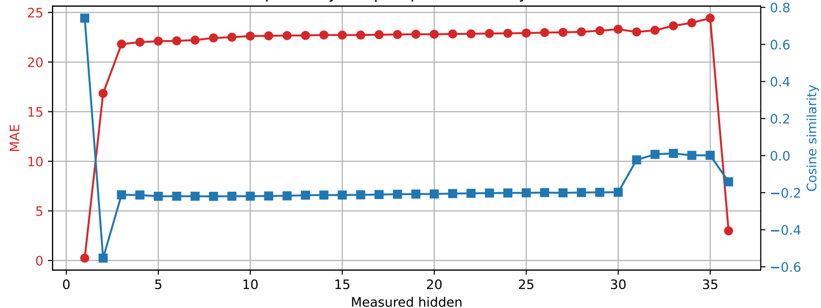
Qwen2.5-3B | Prompt 1 Spared layer 7 | Unquantized vs hybrid
