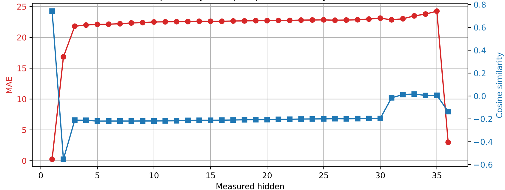
Qwen2.5-3B | Prompt 1 Spared layer 25 | Unquantized vs hybrid
