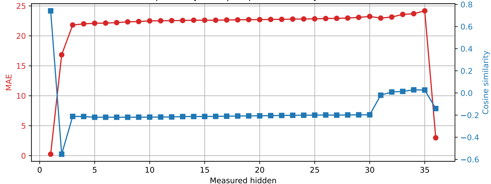
Qwen2.5-3B | Prompt 1 Spared layer 33 | Unquantized vs hybrid
