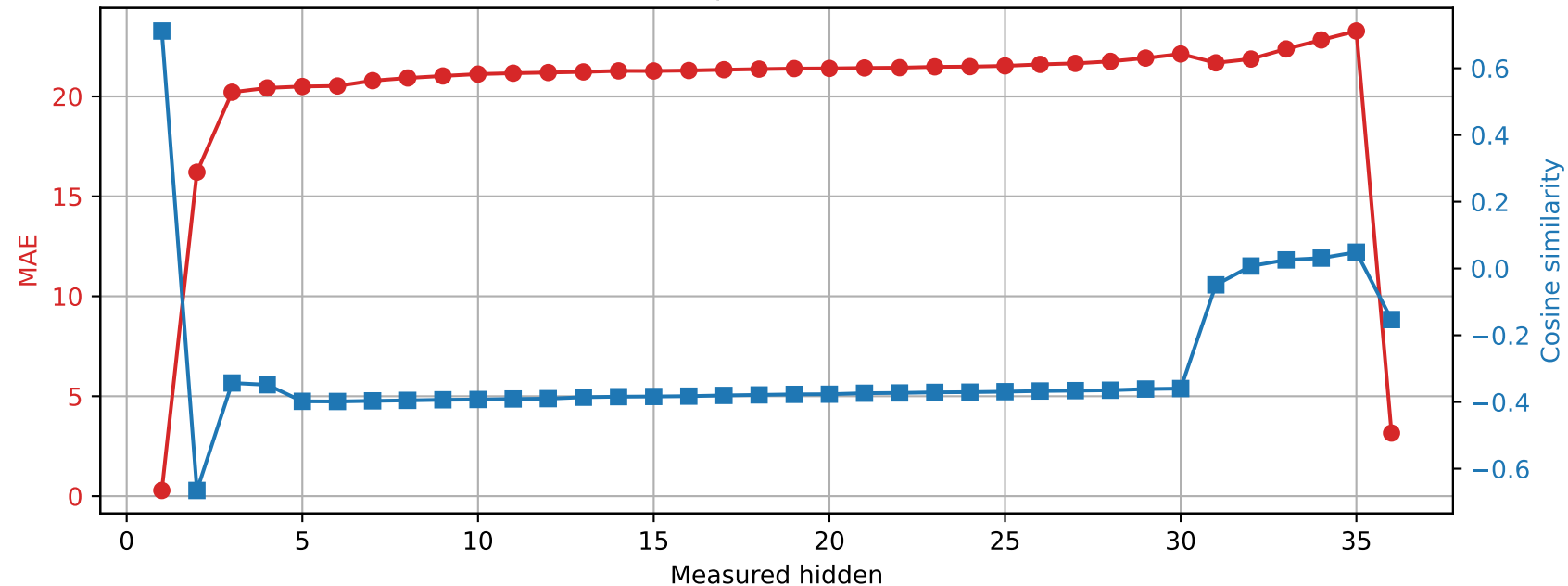
Qwen2.5-3B | Prompt 2 Spared layer 5 | Unquantized vs hybrid
