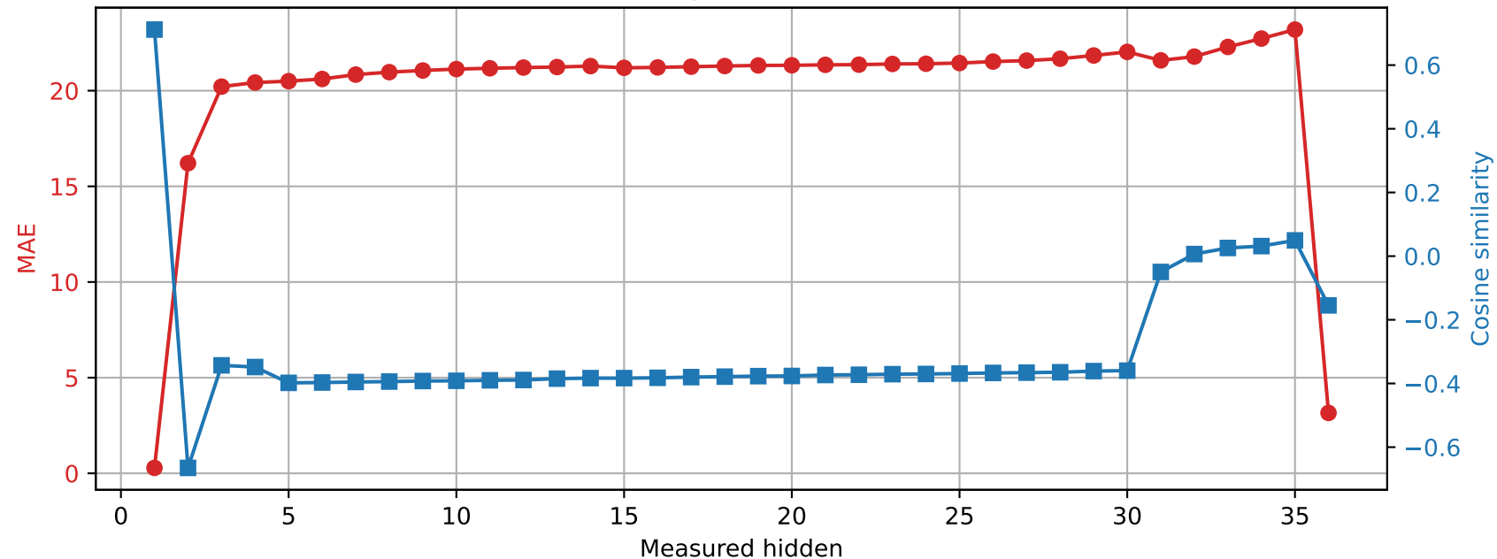
Qwen2.5-3B | Prompt 2 Spared layer 14 | Unquantized vs hybrid
