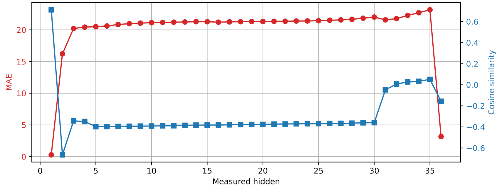
Qwen2.5-3B | Prompt 2 Spared layer 15 | Unquantized vs hybrid
