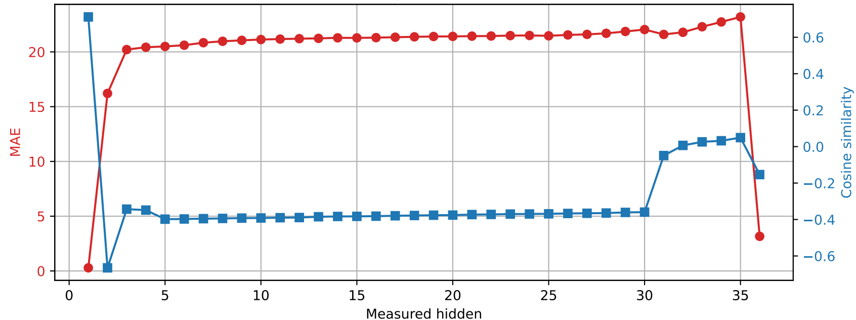
Qwen2.5-3B | Prompt 2 Spared layer 24 | Unquantized vs hybrid
