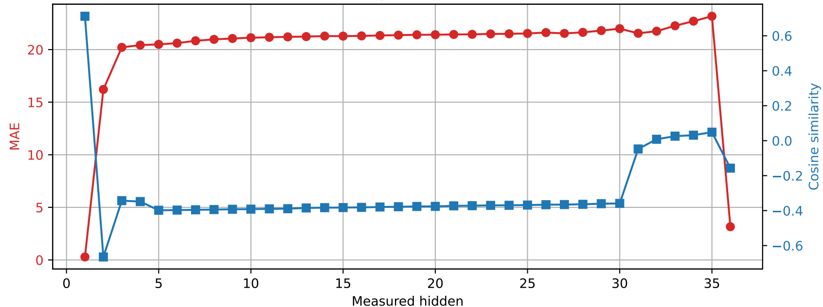
Qwen2.5-3B | Prompt 2 Spared layer 26 | Unquantized vs hybrid
