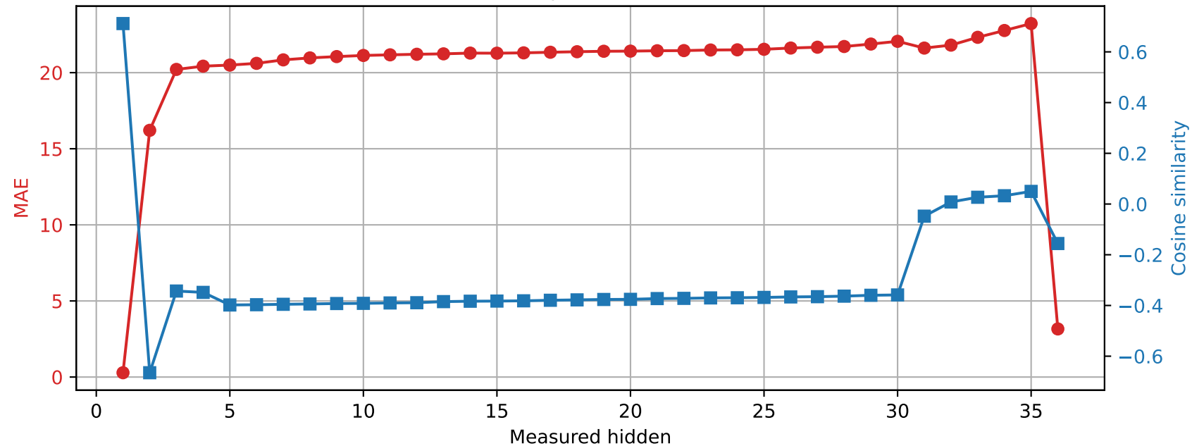
Qwen2.5-3B | Prompt 2 Spared layer 27 | Unquantized vs hybrid
