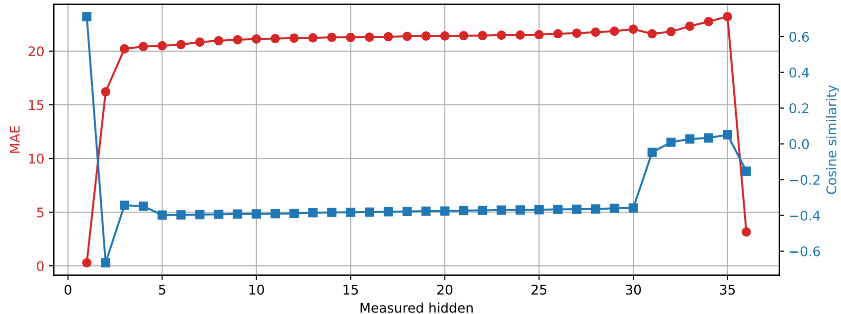
Qwen2.5-3B | Prompt 2 Spared layer 28 | Unquantized vs hybrid
