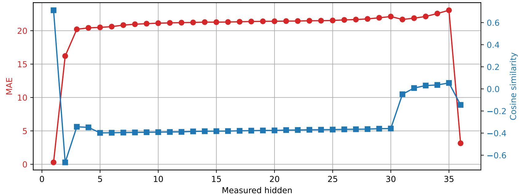
Qwen2.5-3B | Prompt 2 Spared layer 32 | Unquantized vs hybrid
