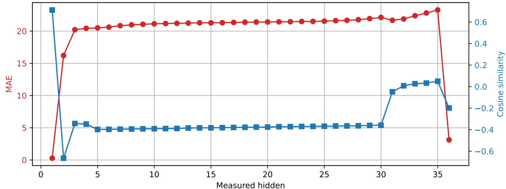
Qwen2.5-3B | Prompt 2 Spared layer 35 | Unquantized vs hybrid
