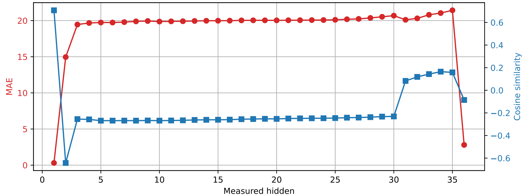
Qwen2.5-3B | Prompt 3 Spared layer 9 | Unquantized vs hybrid
