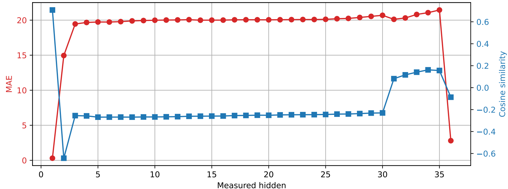
Qwen2.5-3B | Prompt 3 Spared layer 13 | Unquantized vs hybrid
