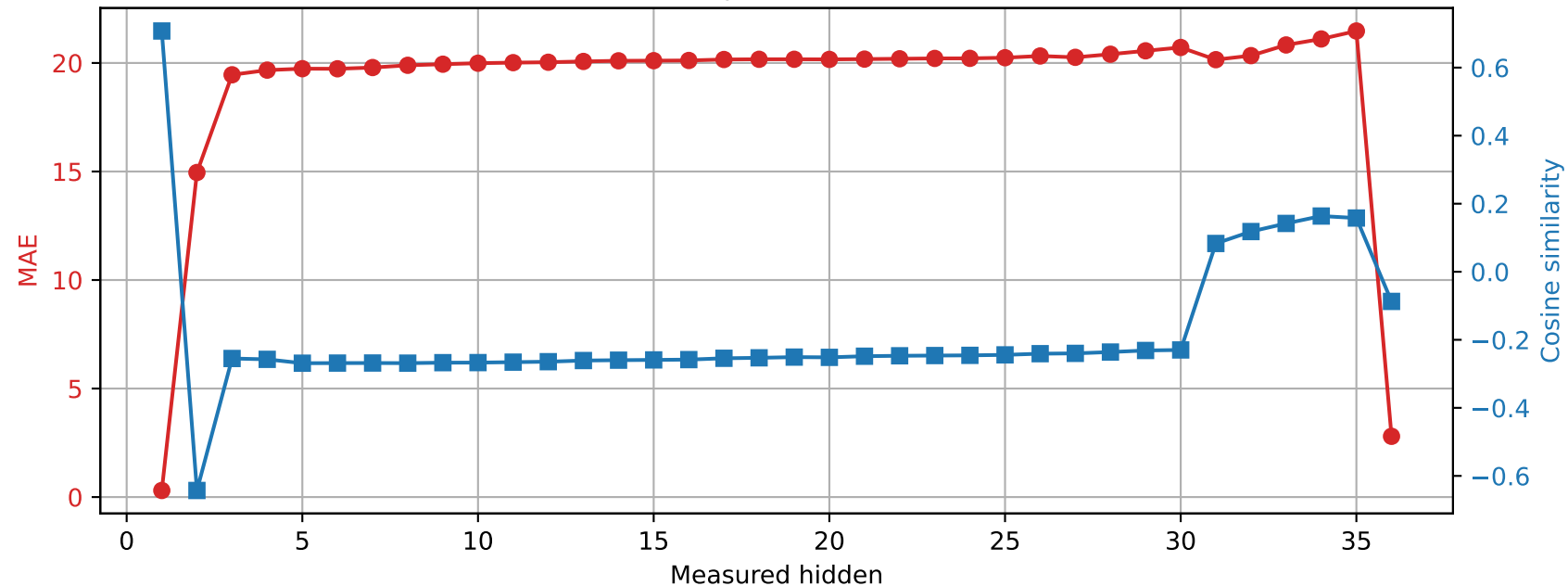
Qwen2.5-3B | Prompt 3 Spared layer 26 | Unquantized vs hybrid
