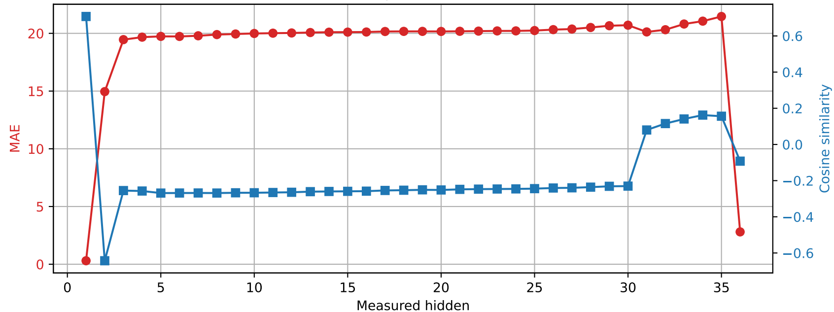
Qwen2.5-3B | Prompt 3 Spared layer 29 | Unquantized vs hybrid
