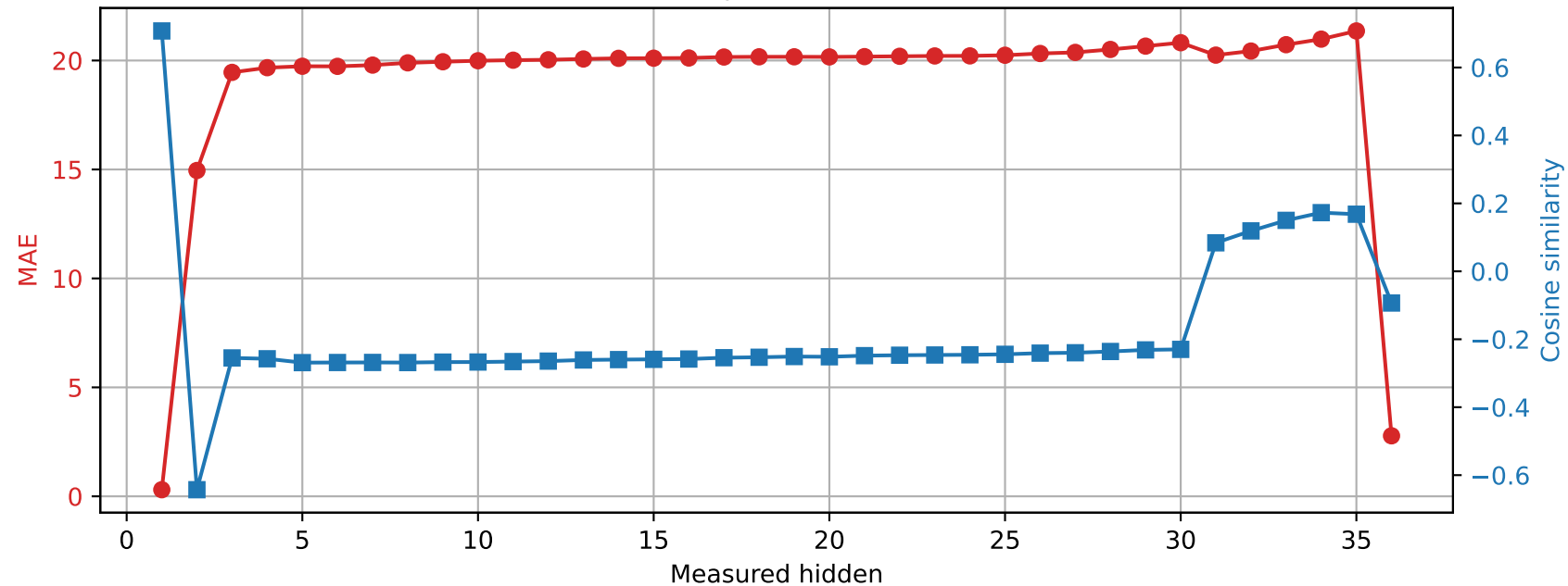
Qwen2.5-3B | Prompt 3 Spared layer 32 | Unquantized vs hybrid
