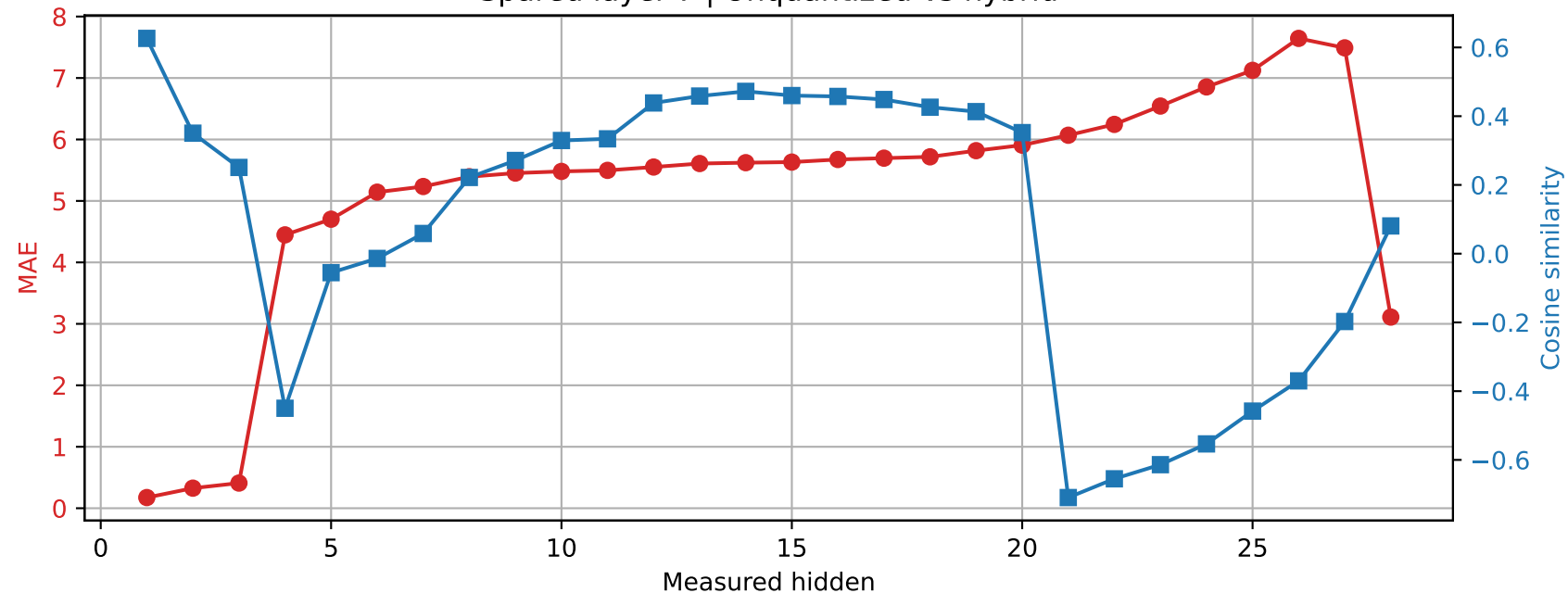
Qwen2.5-7B-Instruct | Prompt 0 Spared layer 7 | Unquantized vs hybrid
