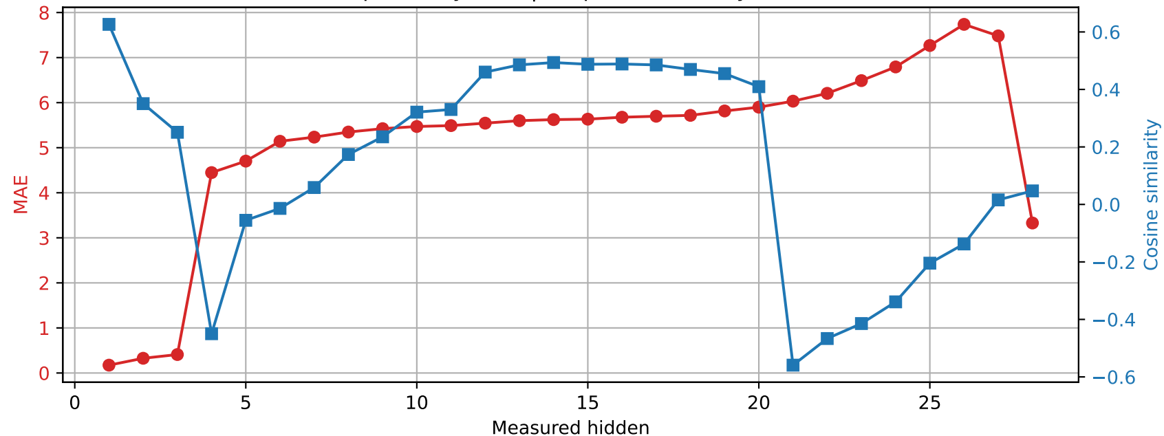
Qwen2.5-7B-Instruct | Prompt 0 Spared layer 24 | Unquantized vs hybrid
