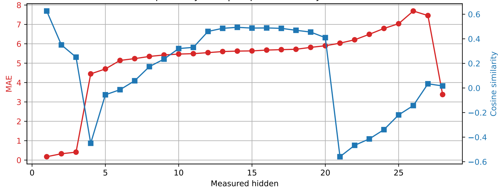
Qwen2.5-7B-Instruct | Prompt 0 Spared layer 25 | Unquantized vs hybrid
