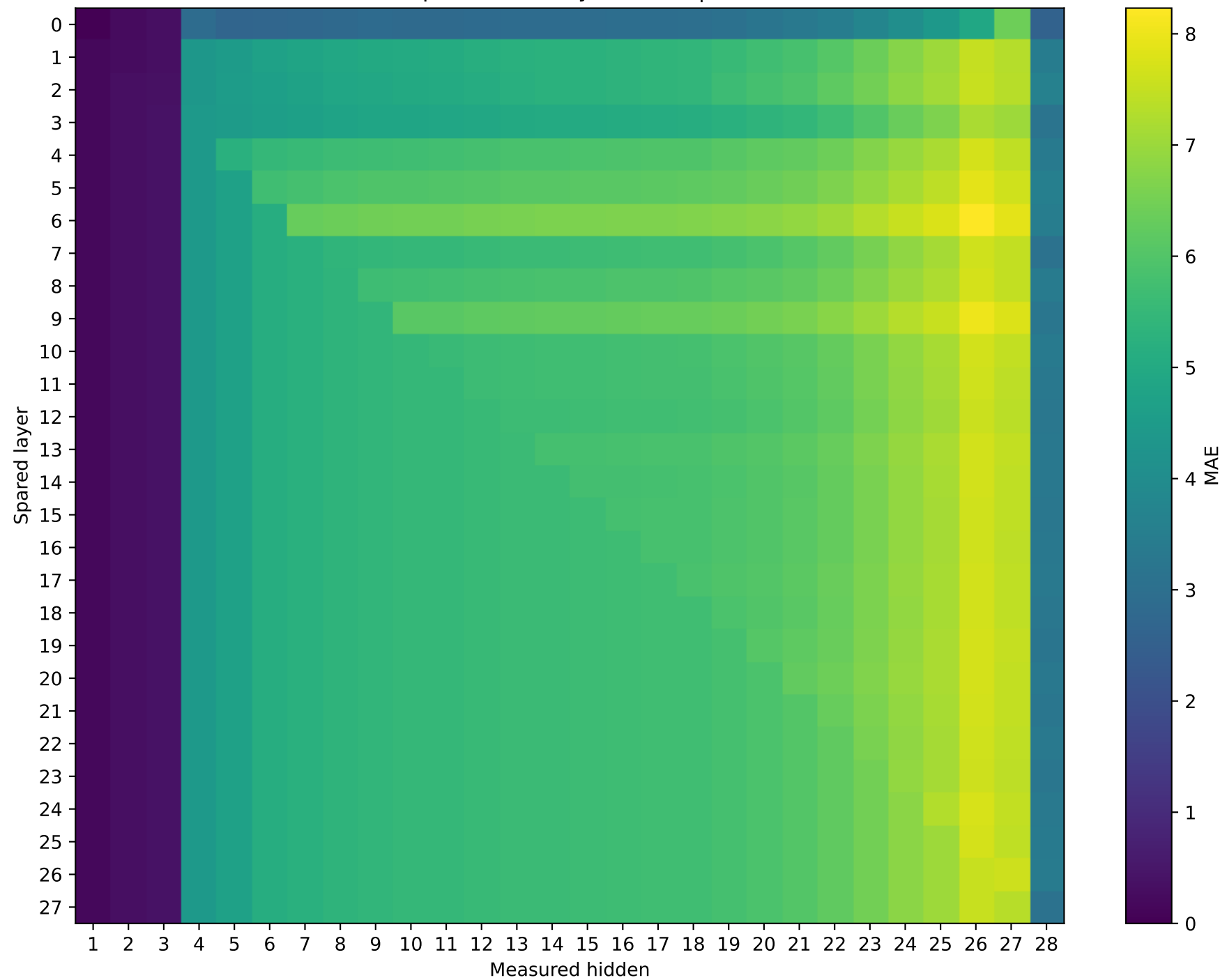
Qwen2.5-7B-Instruct | Prompt 0 Unquantized vs hybrid MAE | int4
