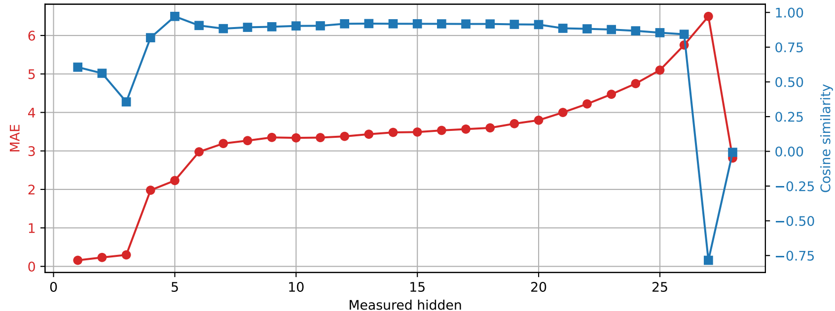
Qwen2.5-7B-Instruct | Prompt 1 Unquantized vs quantized int4
