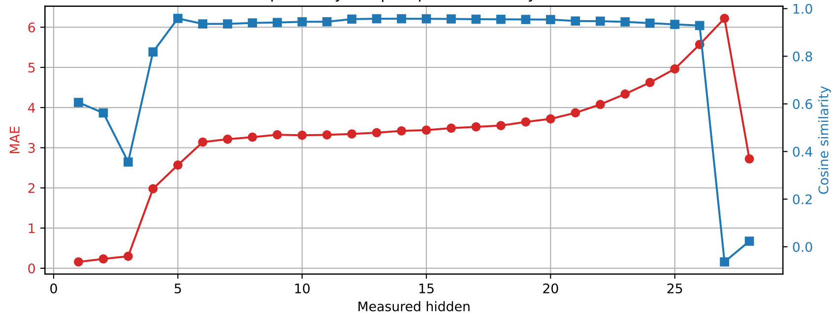
Qwen2.5-7B-Instruct | Prompt 1 Spared layer 4 | Unquantized vs hybrid
