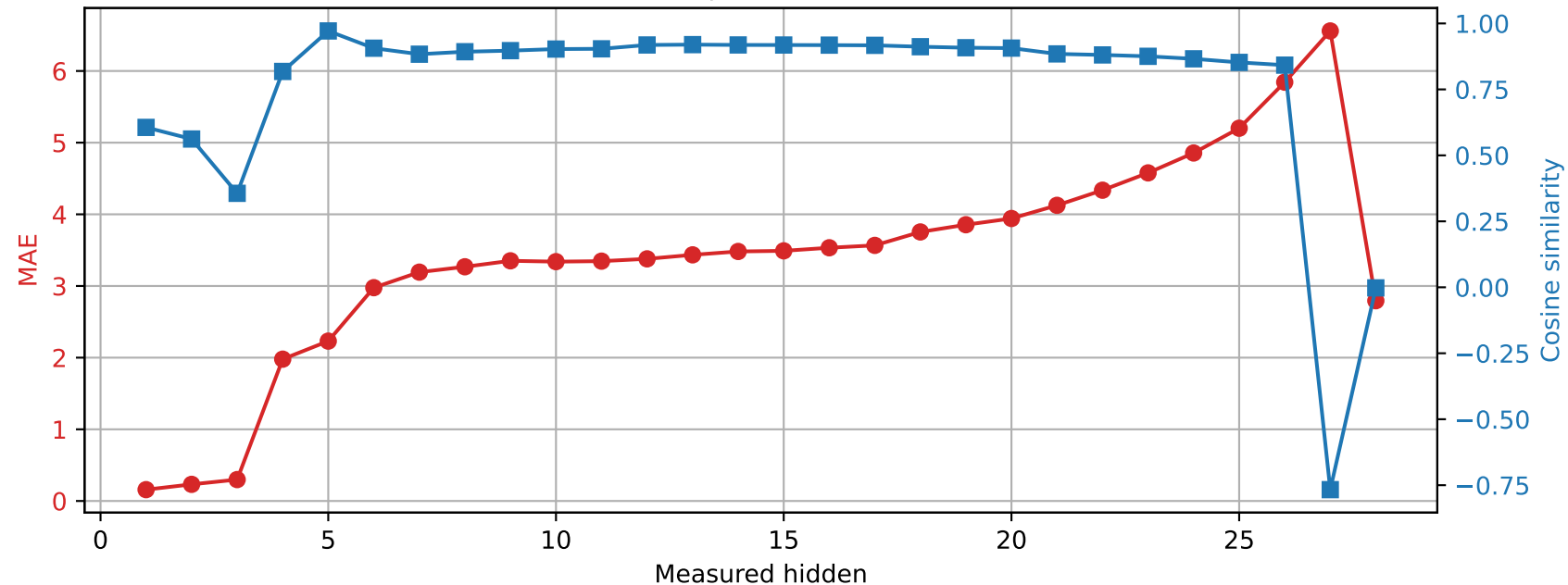
Qwen2.5-7B-Instruct | Prompt 1 Spared layer 17 | Unquantized vs hybrid
