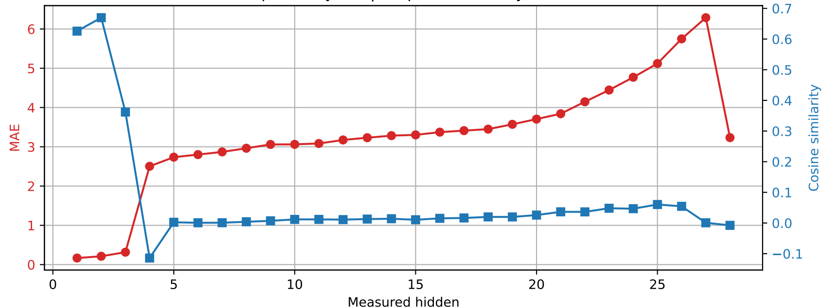
Qwen2.5-7B-Instruct | Prompt 2 Spared layer 1 | Unquantized vs hybrid
