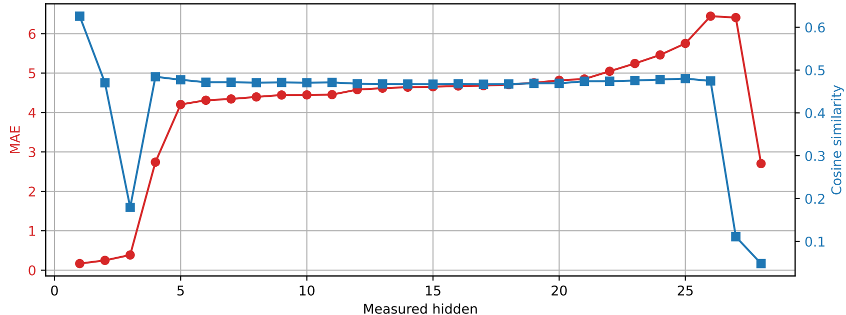
Qwen2.5-7B-Instruct | Prompt 2 Spared layer 4 | Unquantized vs hybrid
