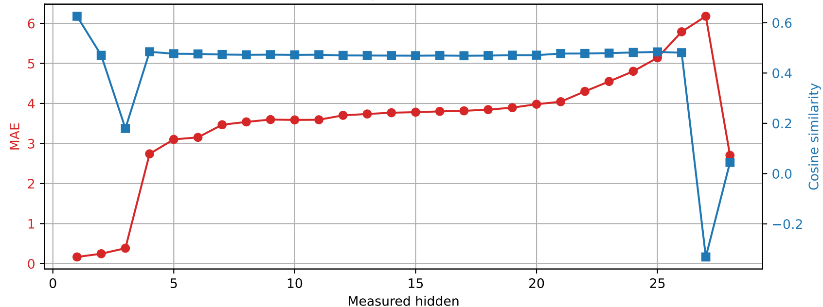
Qwen2.5-7B-Instruct | Prompt 2 Spared layer 6 | Unquantized vs hybrid
