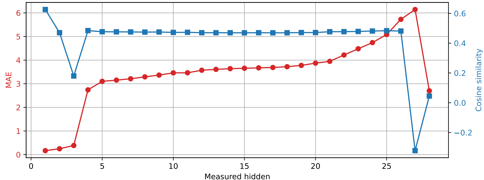
Qwen2.5-7B-Instruct | Prompt 2 Spared layer 9 | Unquantized vs hybrid
