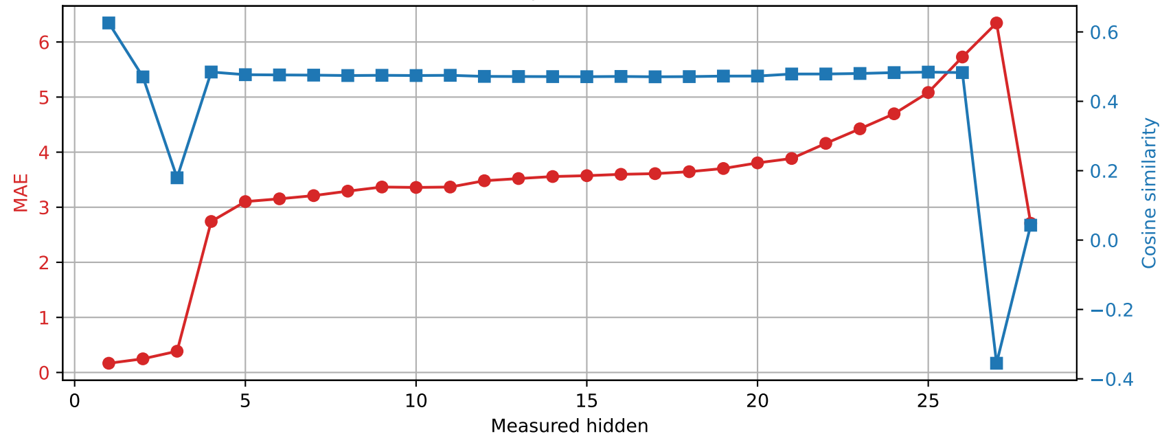
Qwen2.5-7B-Instruct | Prompt 2 Spared layer 24 | Unquantized vs hybrid
