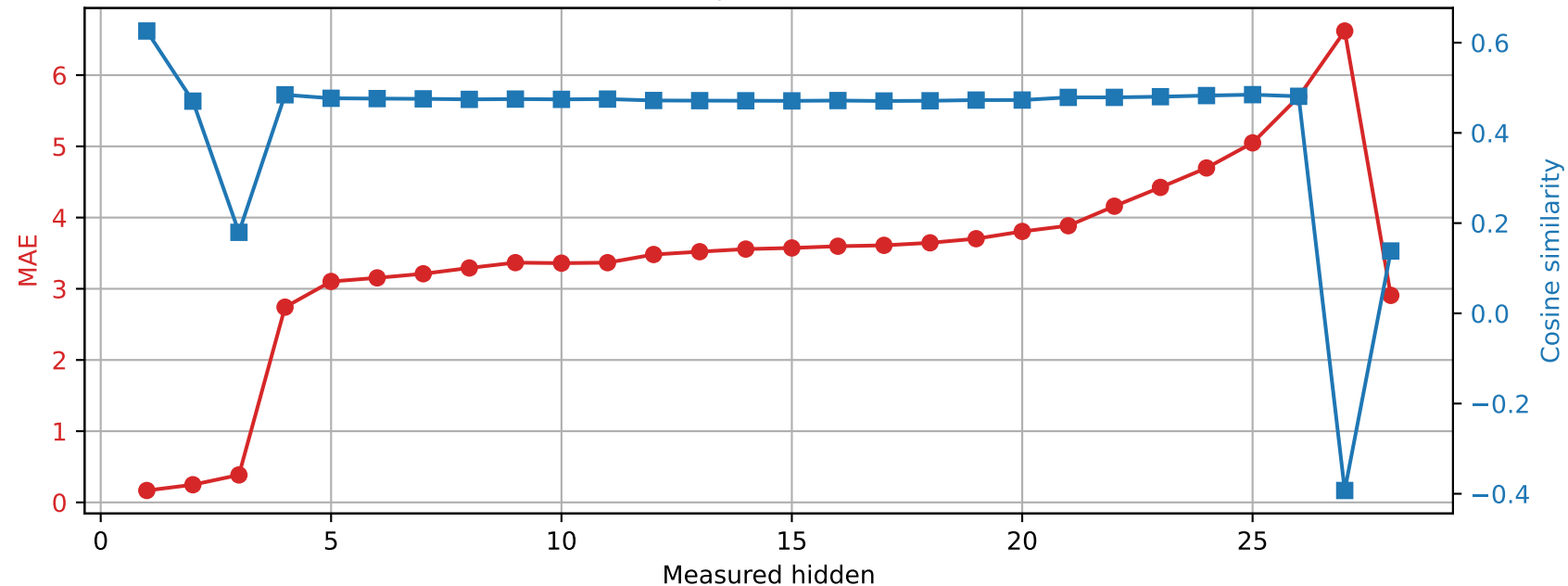
Qwen2.5-7B-Instruct | Prompt 2 Spared layer 27 | Unquantized vs hybrid
