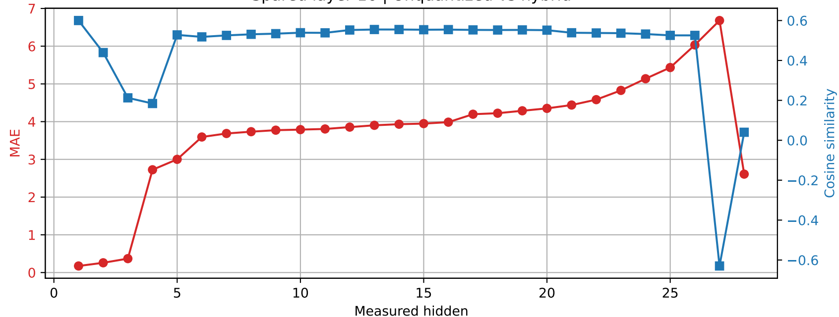
Qwen2.5-7B-Instruct | Prompt 3 Spared layer 16 | Unquantized vs hybrid
