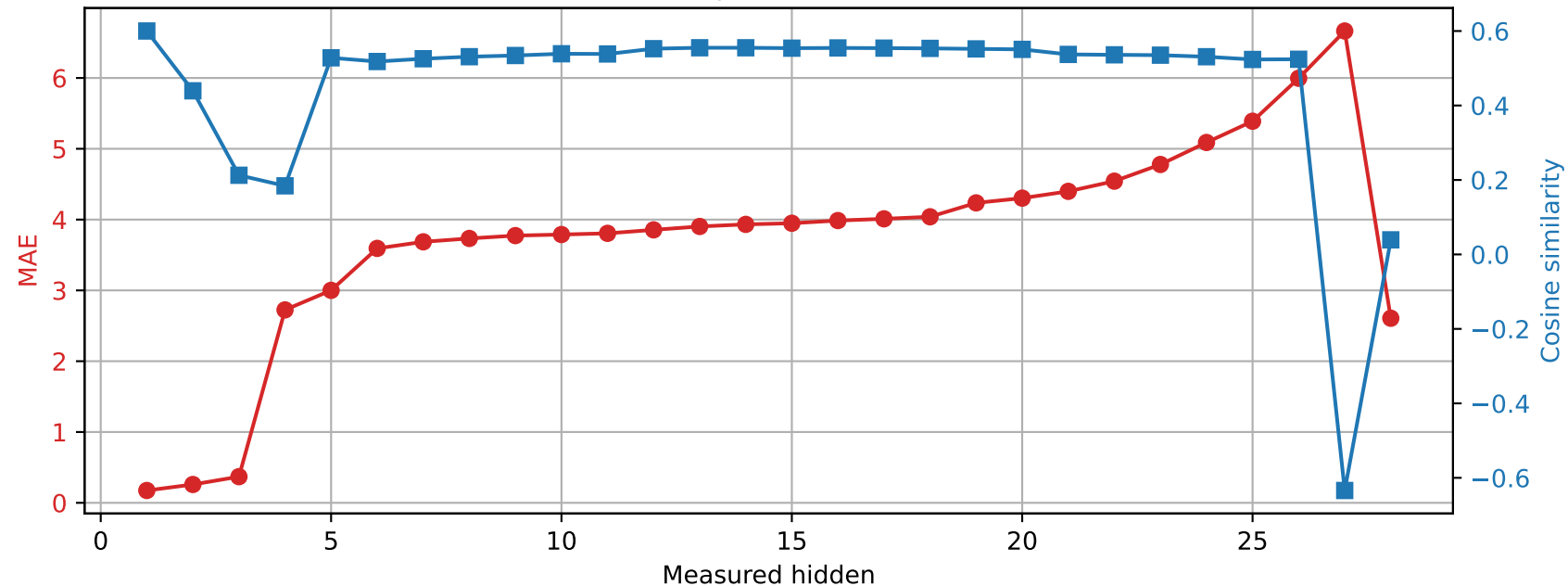
Qwen2.5-7B-Instruct | Prompt 3 Spared layer 18 | Unquantized vs hybrid
