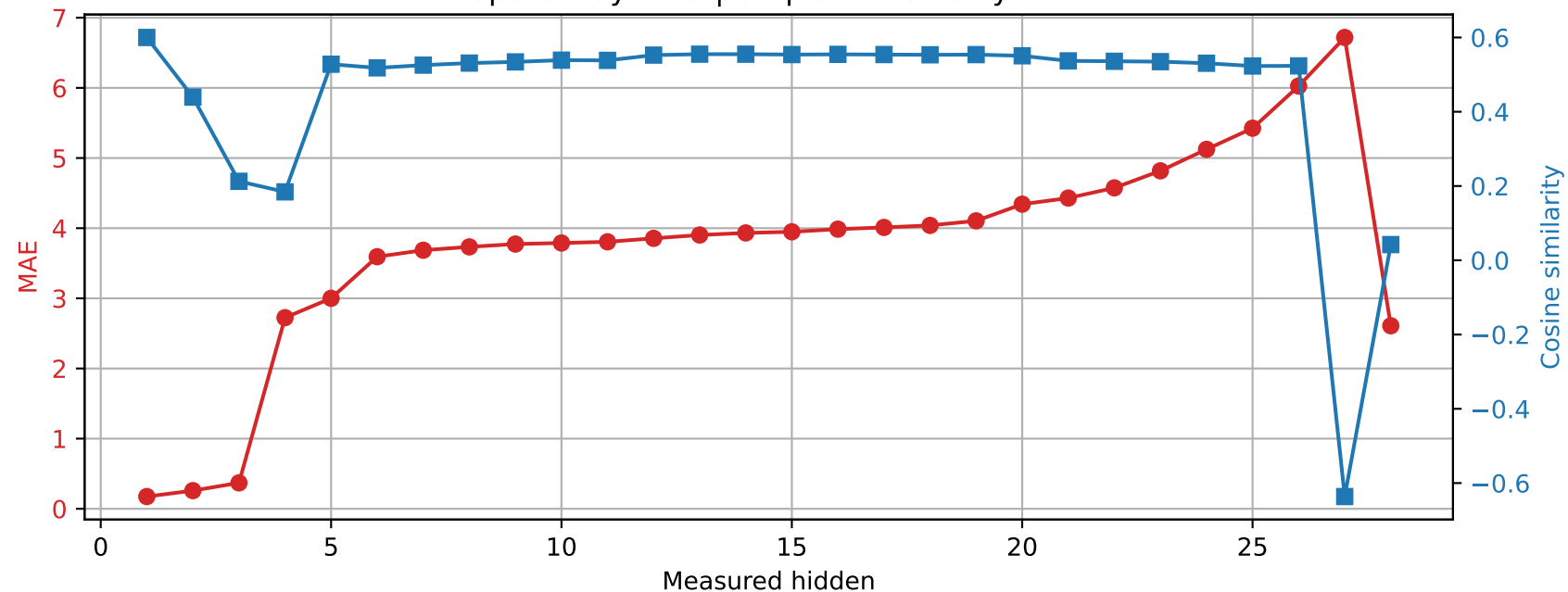
Qwen2.5-7B-Instruct | Prompt 3 Spared layer 19 | Unquantized vs hybrid
