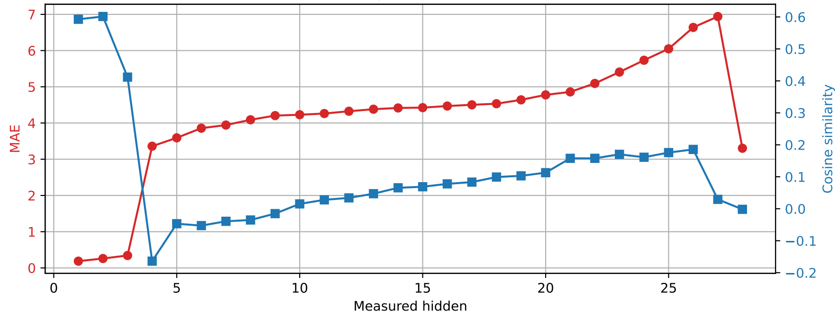
Qwen2.5-7B-Instruct | Prompt 4 Spared layer 1 | Unquantized vs hybrid
