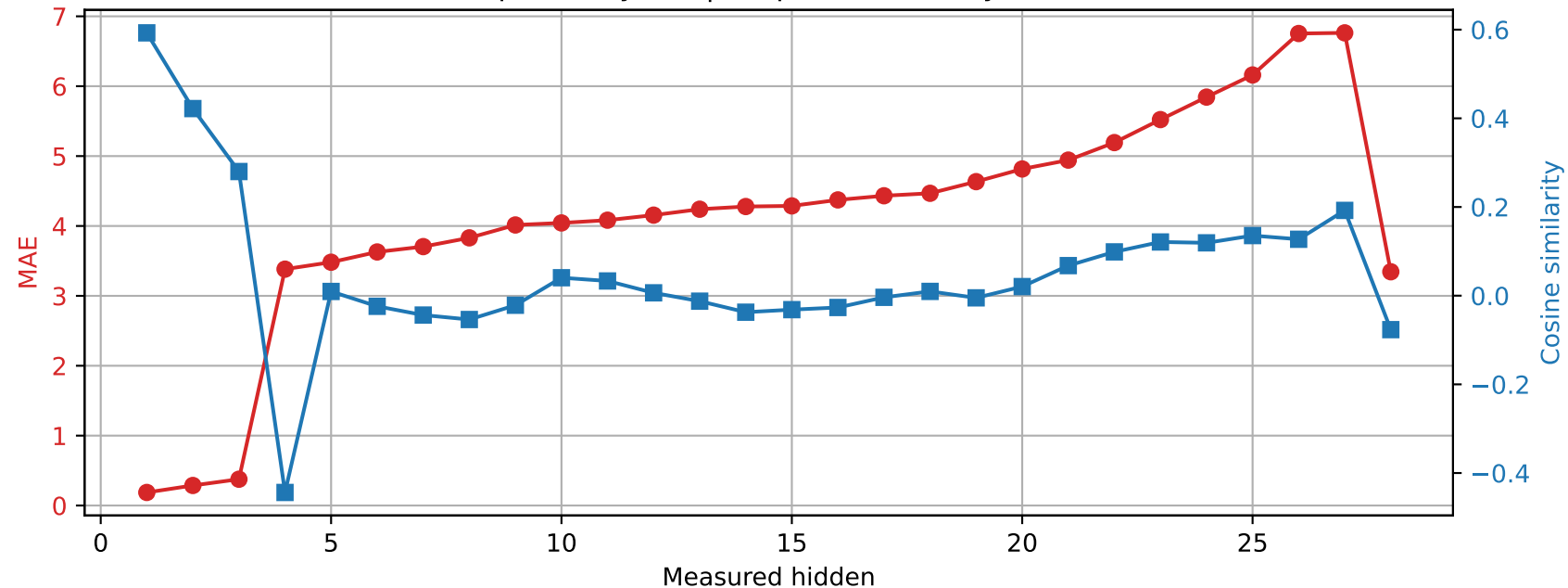
Qwen2.5-7B-Instruct | Prompt 4 Spared layer 8 | Unquantized vs hybrid
