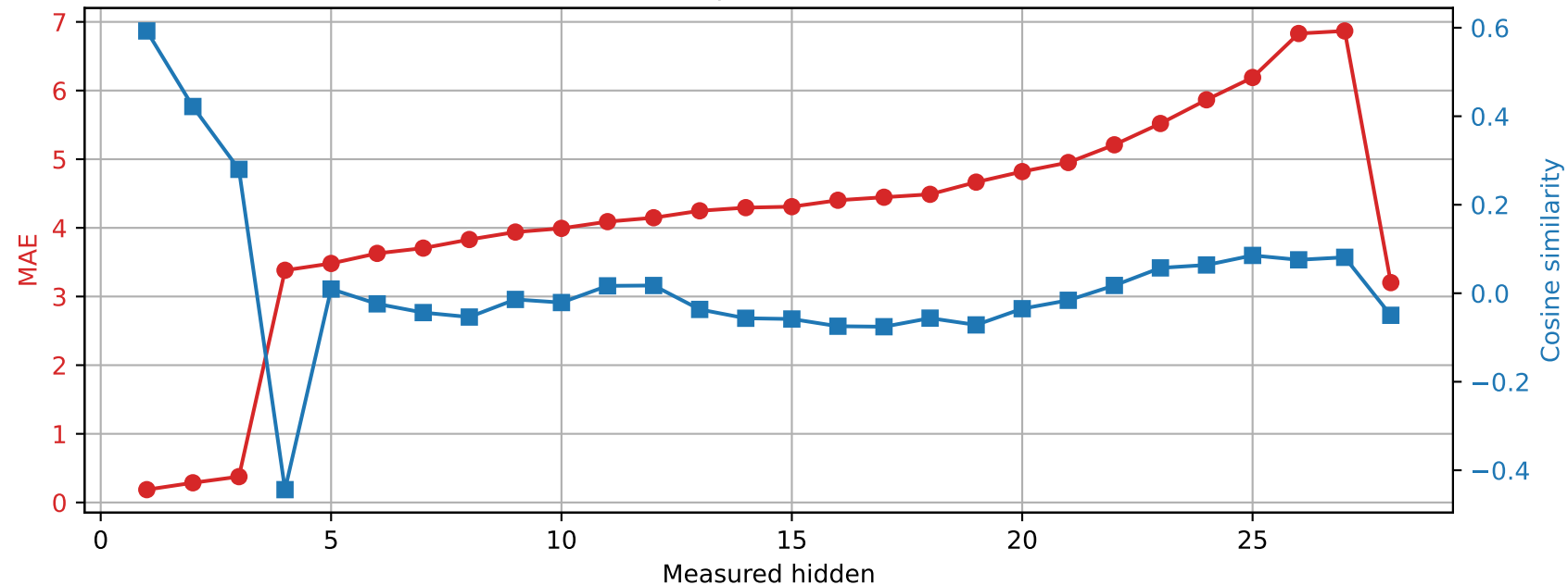
Qwen2.5-7B-Instruct | Prompt 4 Spared layer 10 | Unquantized vs hybrid
