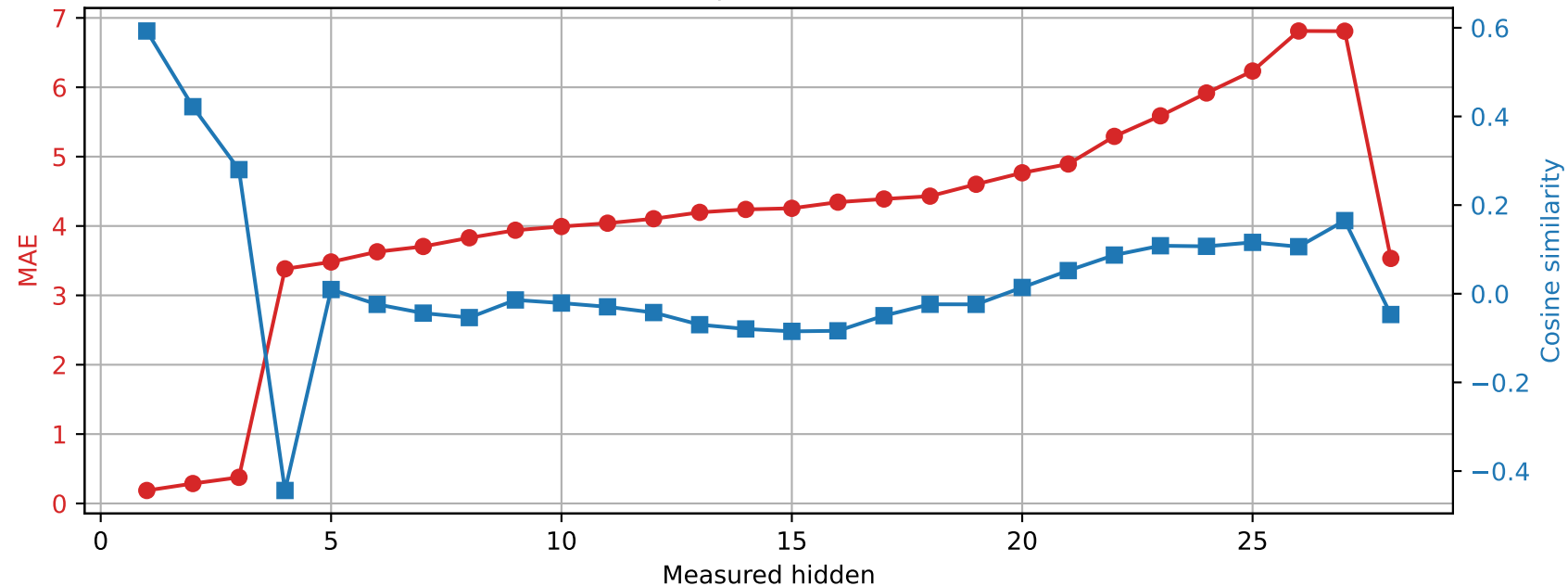
Qwen2.5-7B-Instruct | Prompt 4 Spared layer 21 | Unquantized vs hybrid
