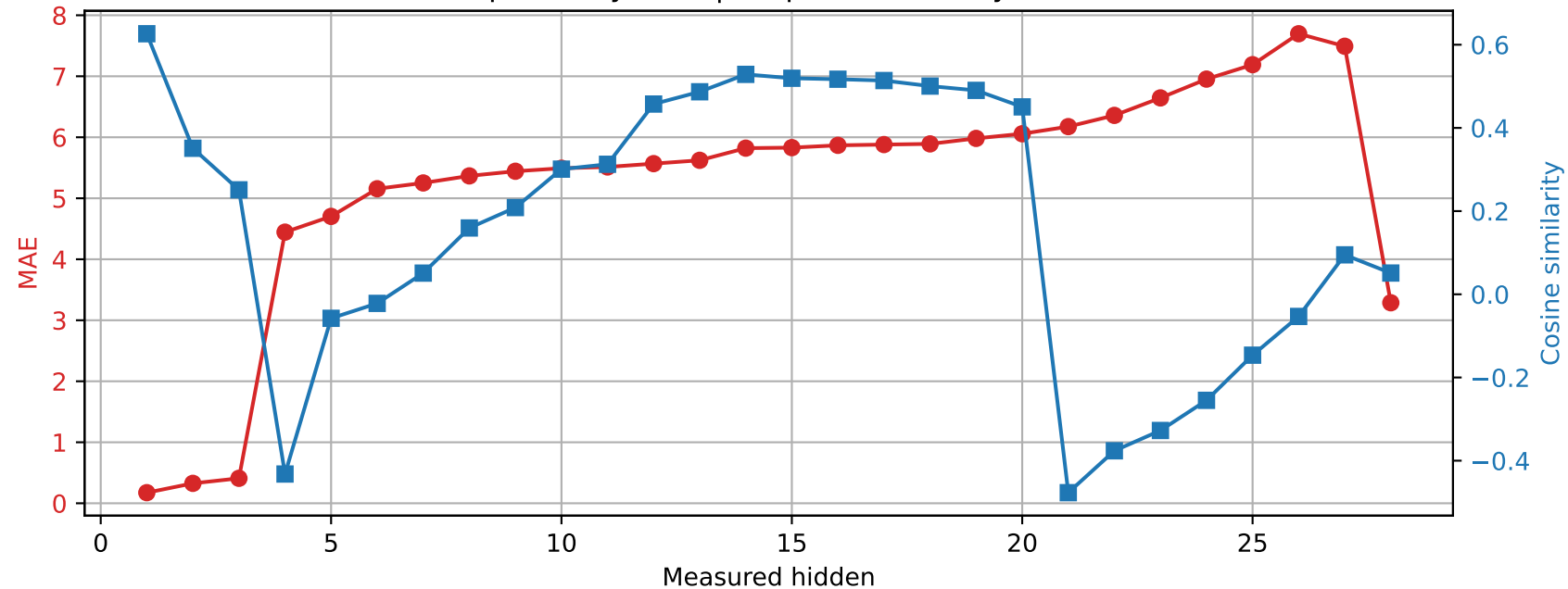
Qwen2.5-7B-Instruct | Prompt 0 Spared layer 13 | Unquantized vs hybrid
