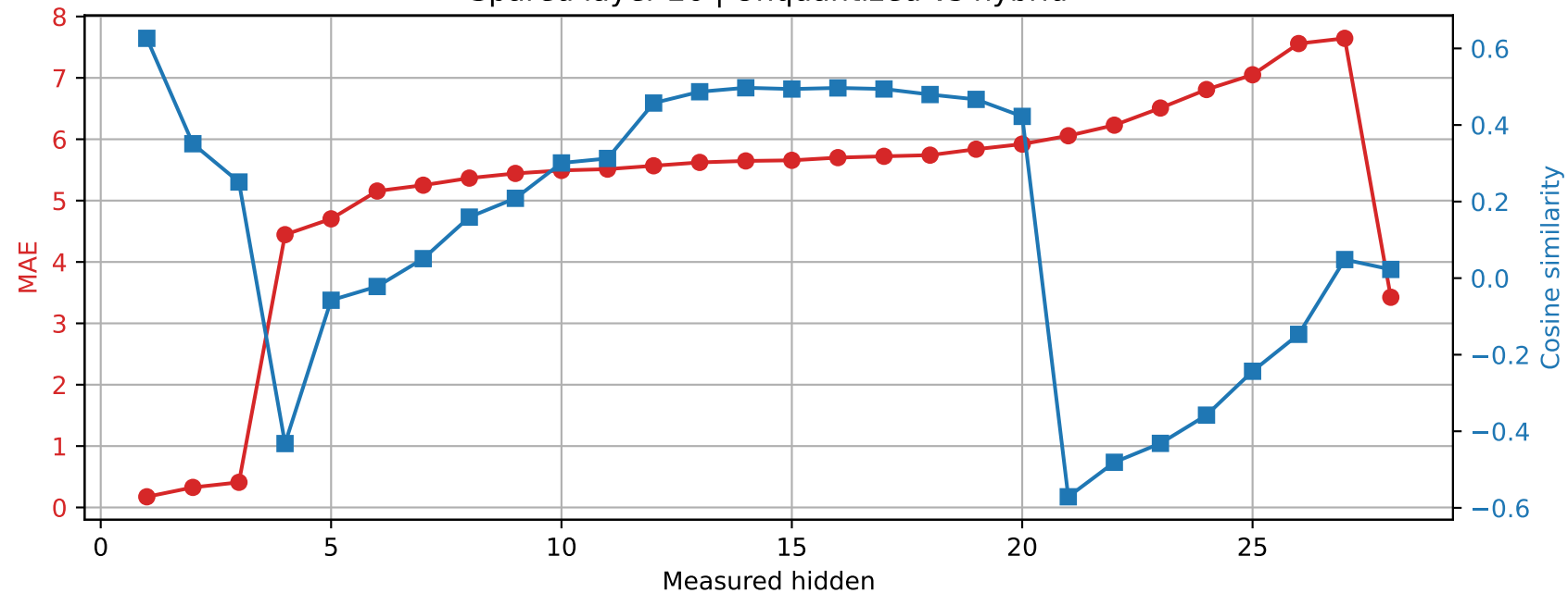
Qwen2.5-7B-Instruct | Prompt 0 Spared layer 26 | Unquantized vs hybrid
