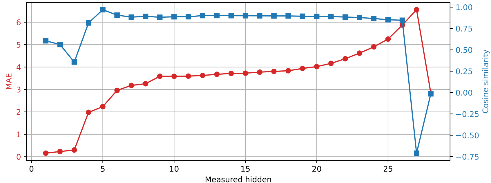
Qwen2.5-7B-Instruct | Prompt 1 Spared layer 8 | Unquantized vs hybrid
