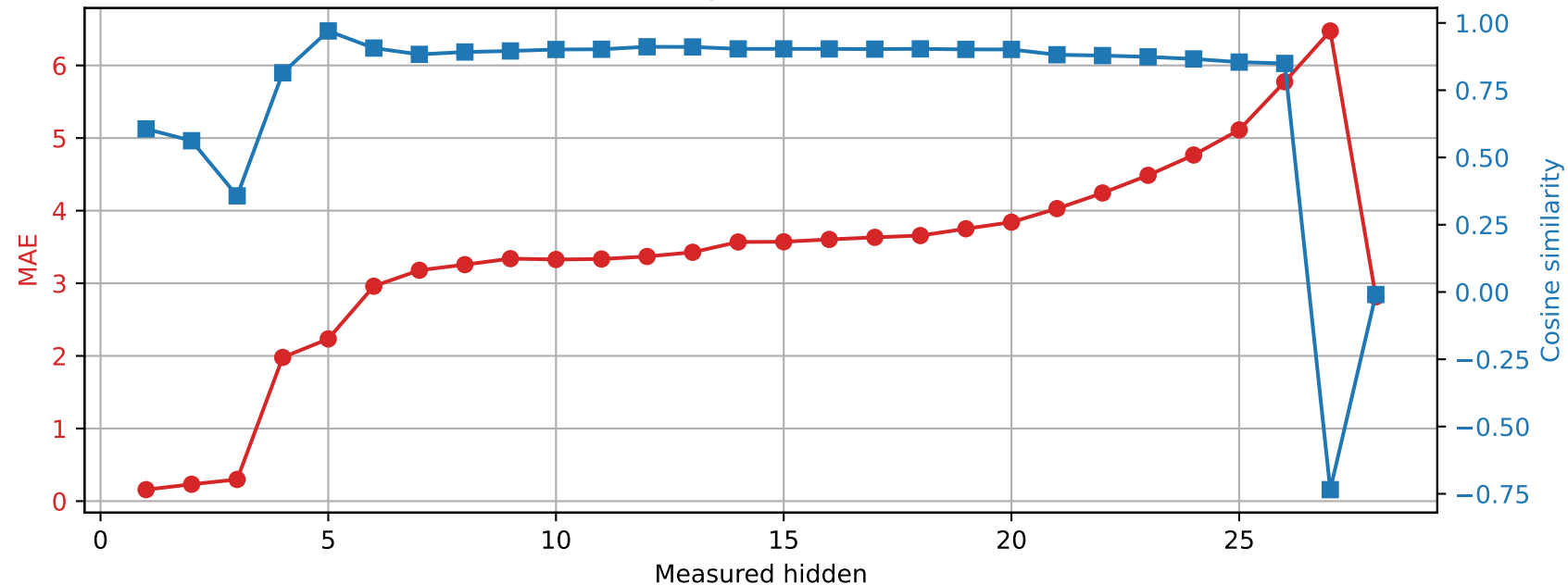
Qwen2.5-7B-Instruct | Prompt 1 Spared layer 13 | Unquantized vs hybrid
