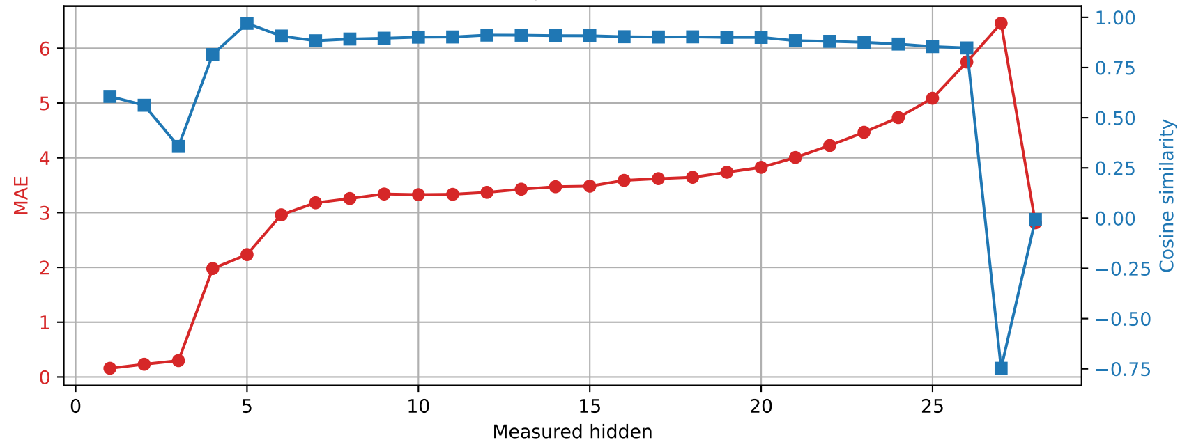
Qwen2.5-7B-Instruct | Prompt 1 Spared layer 15 | Unquantized vs hybrid
