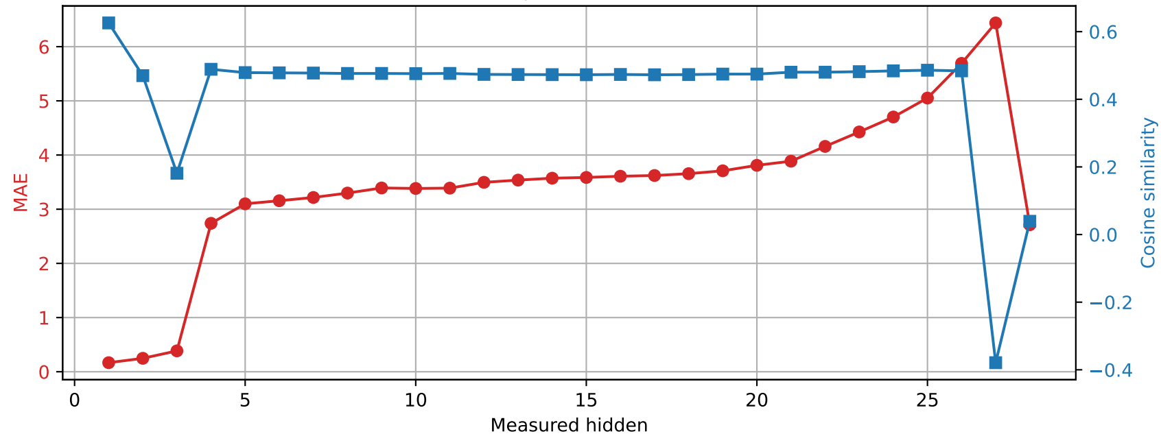
Qwen2.5-7B-Instruct | Prompt 2 Spared layer 8 | Unquantized vs hybrid
