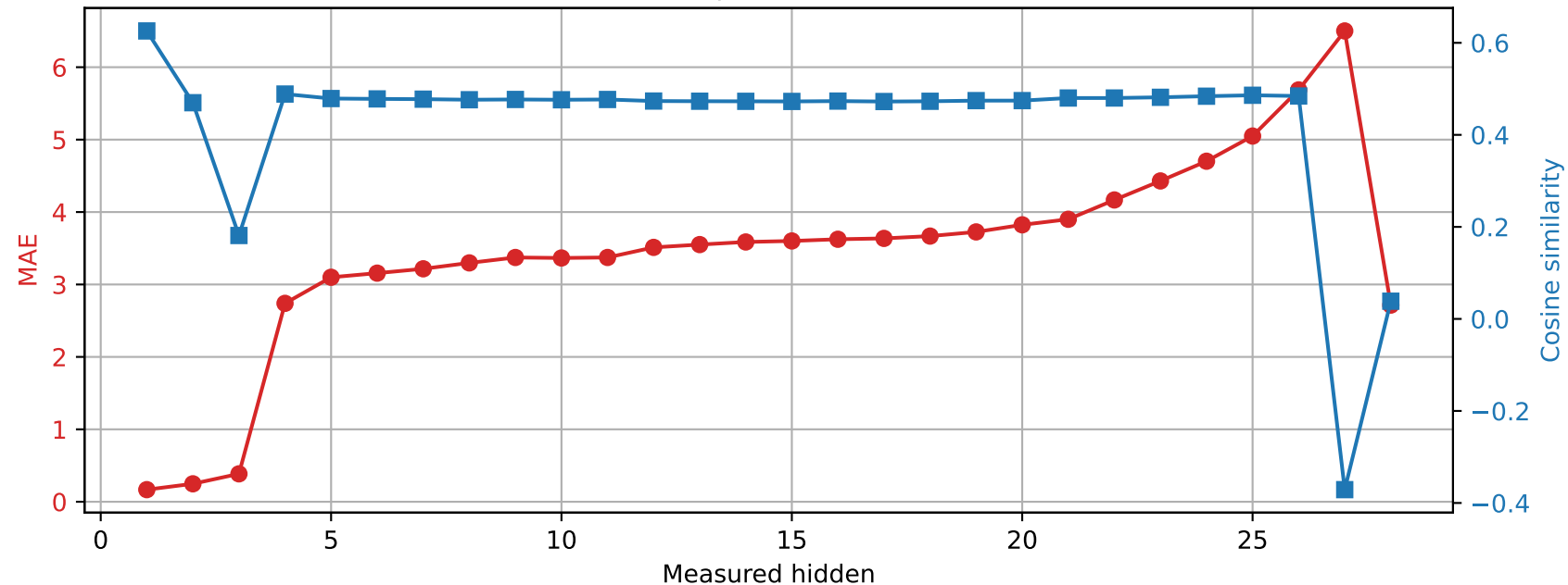
Qwen2.5-7B-Instruct | Prompt 2 Spared layer 11 | Unquantized vs hybrid
