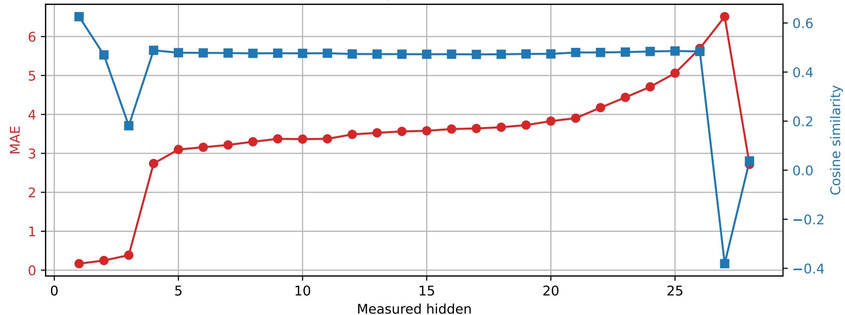
Qwen2.5-7B-Instruct | Prompt 2 Spared layer 15 | Unquantized vs hybrid
