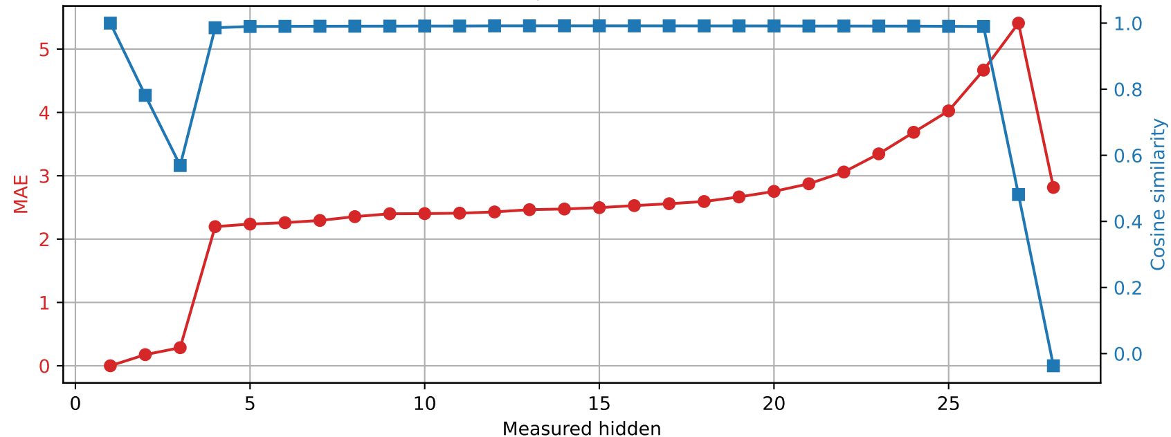
Qwen2.5-7B-Instruct | Prompt 3 Spared layer 0 | Unquantized vs hybrid
