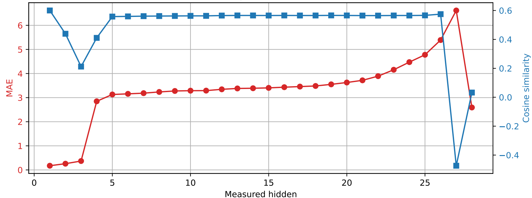
Qwen2.5-7B-Instruct | Prompt 3 Spared layer 3 | Unquantized vs hybrid
